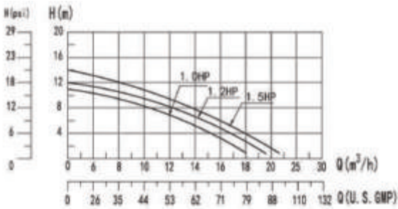
性能曲线Performance curve
